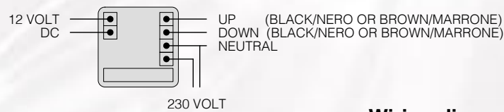
Wiring diagram
