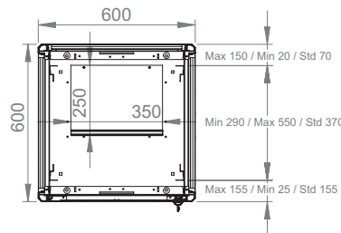
Max/std/min equipment mounting distance
