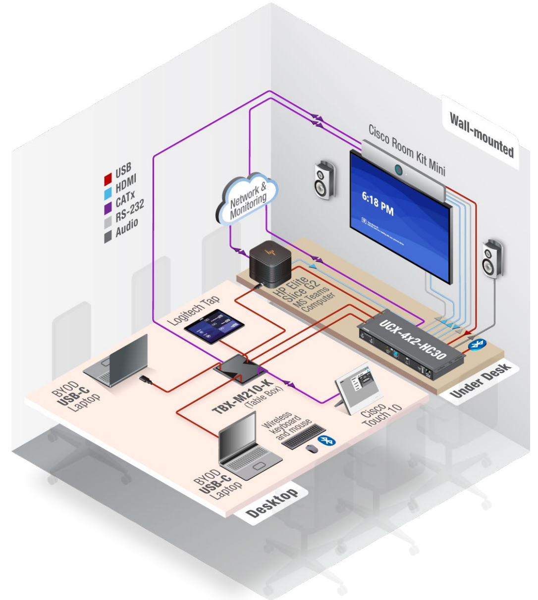
UCX-4x2-HC30 - Example 2.
