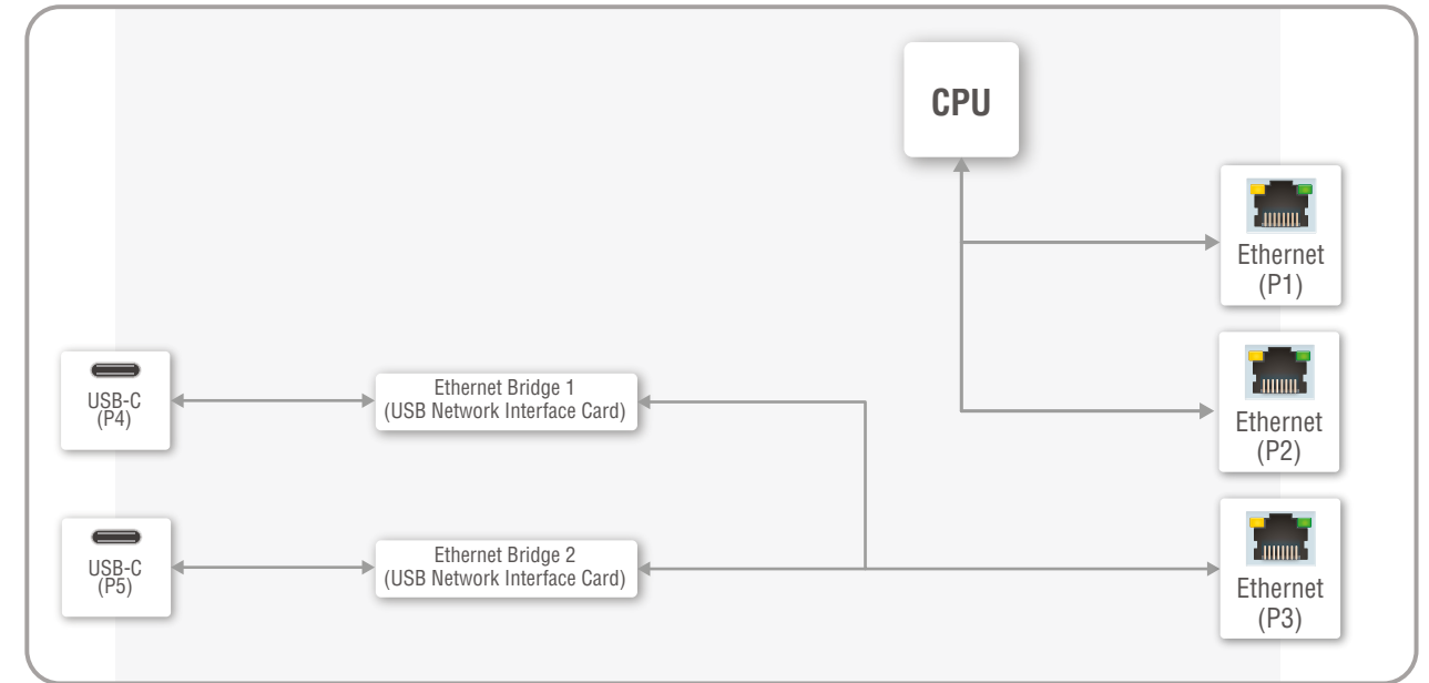
Separated BYOD VLAN preset in UCX-4x2-HC30(D)
