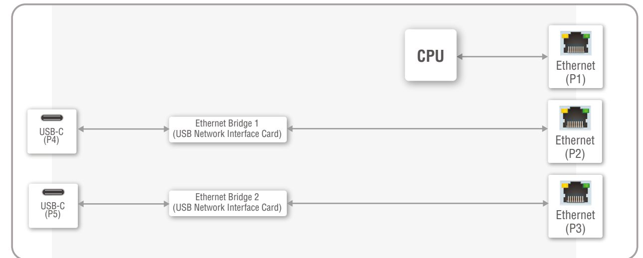
Dedicated VLAN preset in UCX-4x2-HC30(D)
