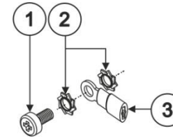
Figure 3: Grounding Connection Components
