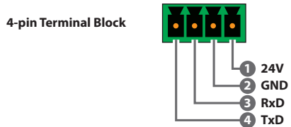
RS-232 Port 2 (HDBaseT extension)
