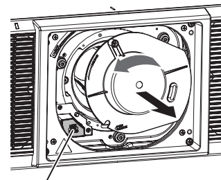
Lens release button
